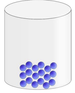
Solid
