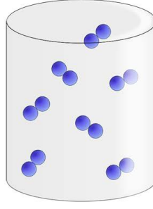
Gas
